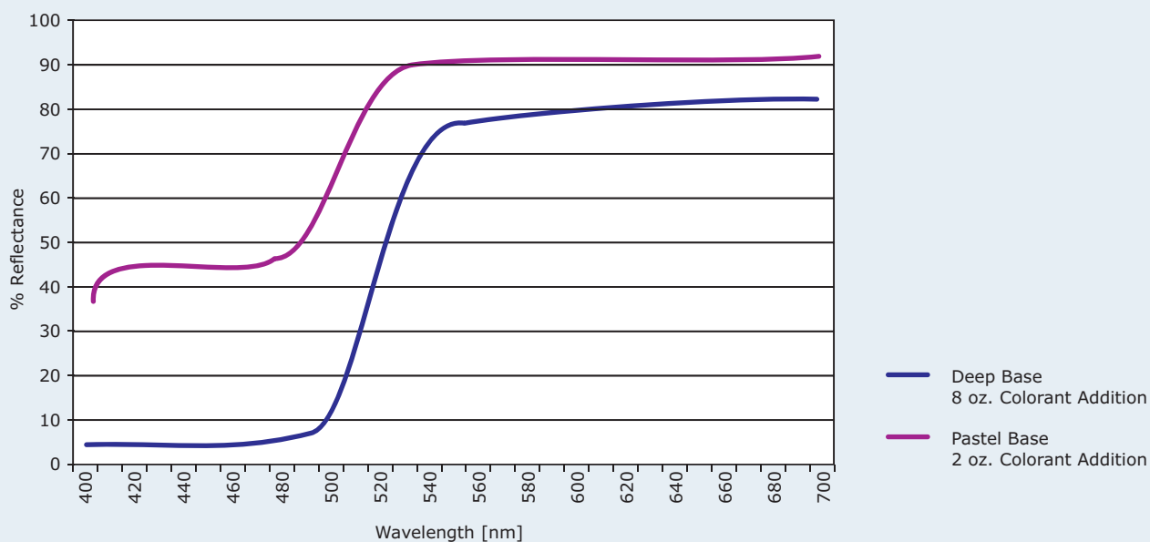
Spectral Curves for HEUCOTINT YU13003 Organic Yellow AXX
