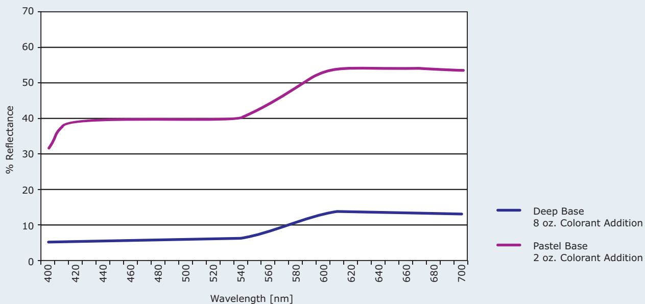
Spectral Curves for HEUCOTINT XU17003 Brown Oxide I
