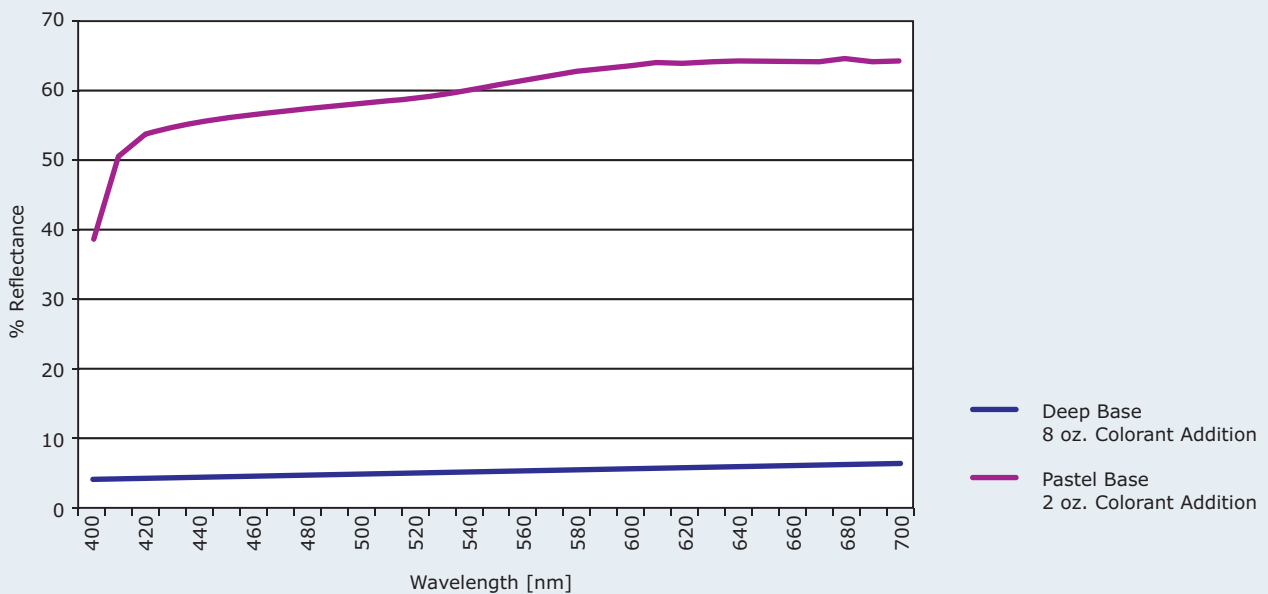
Spectral Curves for HEUCOTINT XU17002 Raw Umber L
