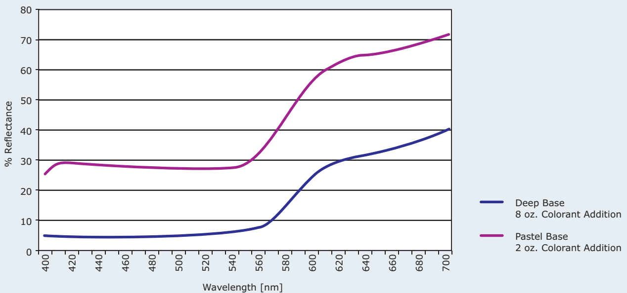
Spectral Curves for HEUCOTINT RU11003 Red Oxide F
