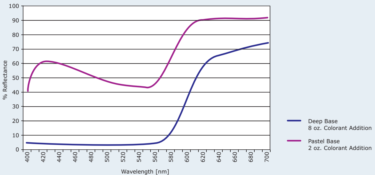
Spectral Curves for HEUCOTINT RU11002 Organic Red
