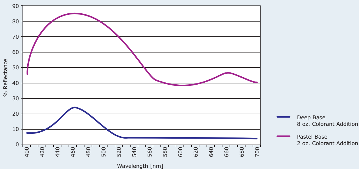
Spectral Curves for HEUCOTINT BU15001 Phthalo Blue E
